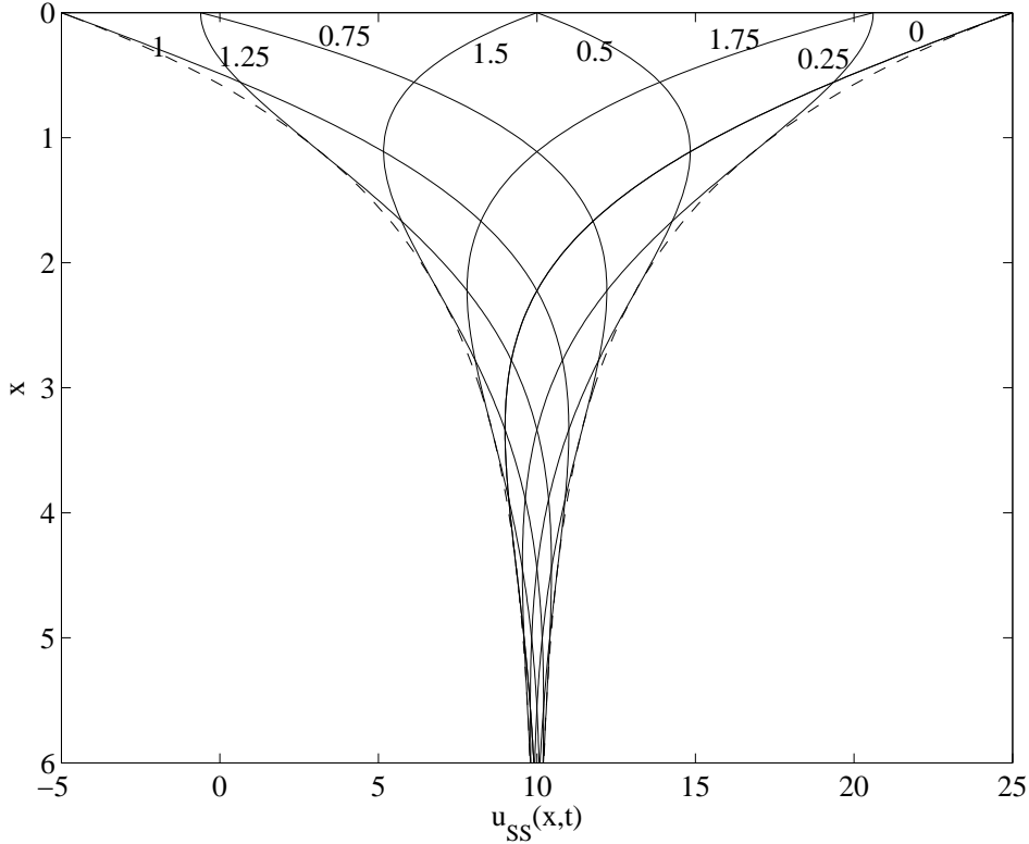
Figure 5: Plot of u_{SS}(x, t) for the first 6 m at various times. Numbers in figure indicate \omega t/\pi .
