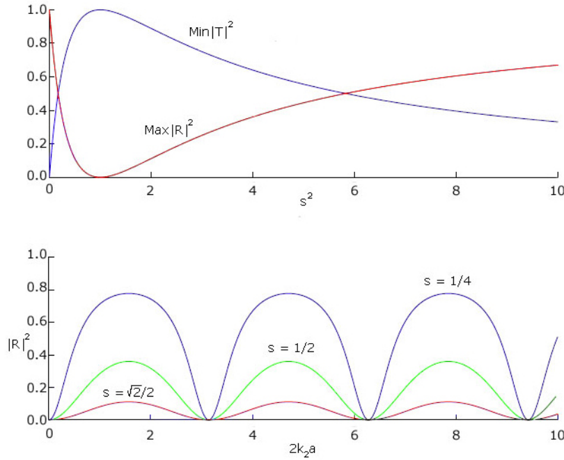
Figure 11: Transmission and reflection coefficients for a rectangular shelf. From Mei, C.C., Applied Dynamics of Ocean Surface Waves .
