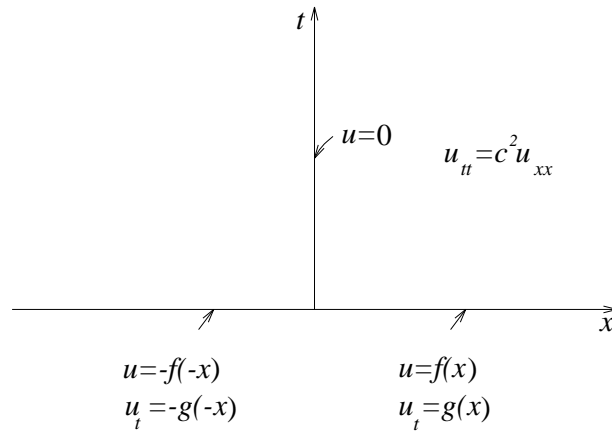
Figure 5: Initial-boundary-value problem and the mirror reflection
